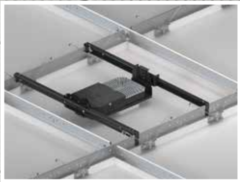
Snap-In Mounting System - Seismically Rated Self Leveling + Centering
